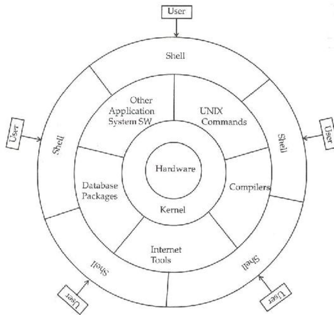
Fig 1.1: Structure of UNIX Operating System
